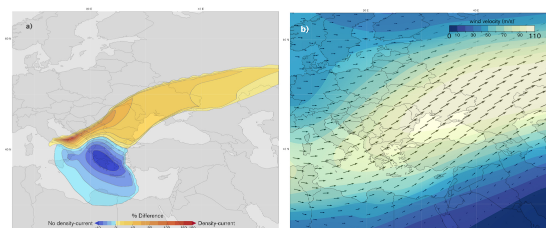
Figure S1. (a) Impact of gravity current on the deposit (variation in %). Positive values show areas where tephra deposition increases when accounting for gravity-current effects; negative indicate lesser tephra deposition. (b) Wind field at ~32 km elevation for the meteorological field that best represents the (unknown) meteorological conditions at the time of the CI eruption (7th December 1991). Figure generated using Autodesk(R) Maya(R).
