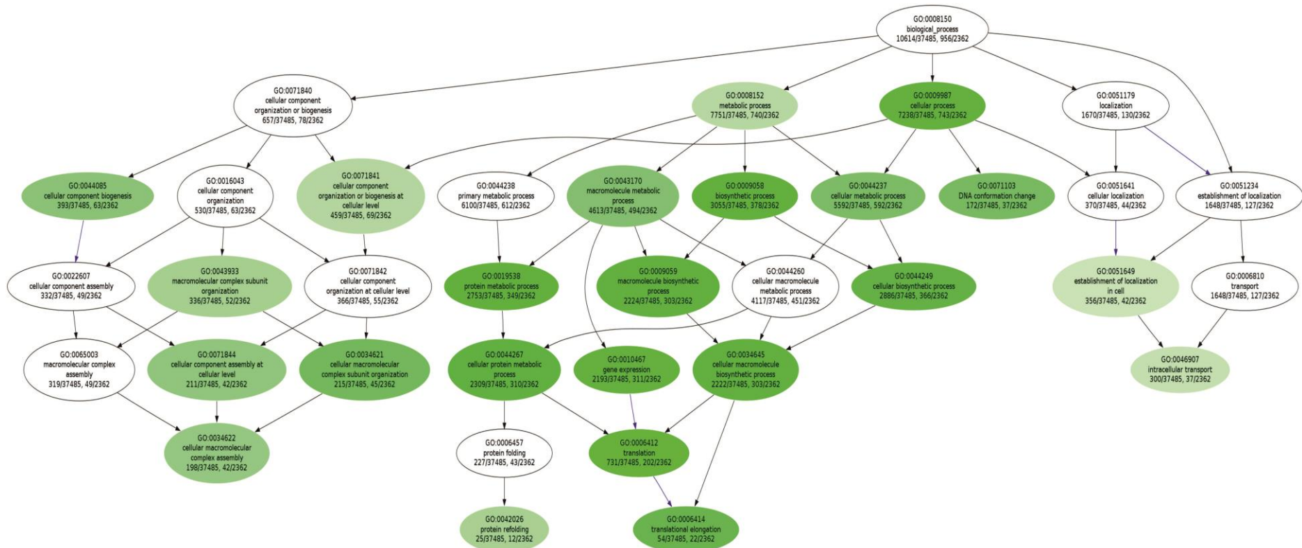
Additional file 15. Gene Ontology categories of GO class “Biological Process” significantly over-represented among transcripts up-regulated by cold treatment in S50676 inbred line. Only the relevant fragment of the GO graph is shown with over-represented categories highlighted. Numbers attributed to a GO term indicate, respectively: total number of proteins described by this GO term in the population/size of the population; number of cold-repressed proteins described by this GO term/total number of cold-repressed proteins.
