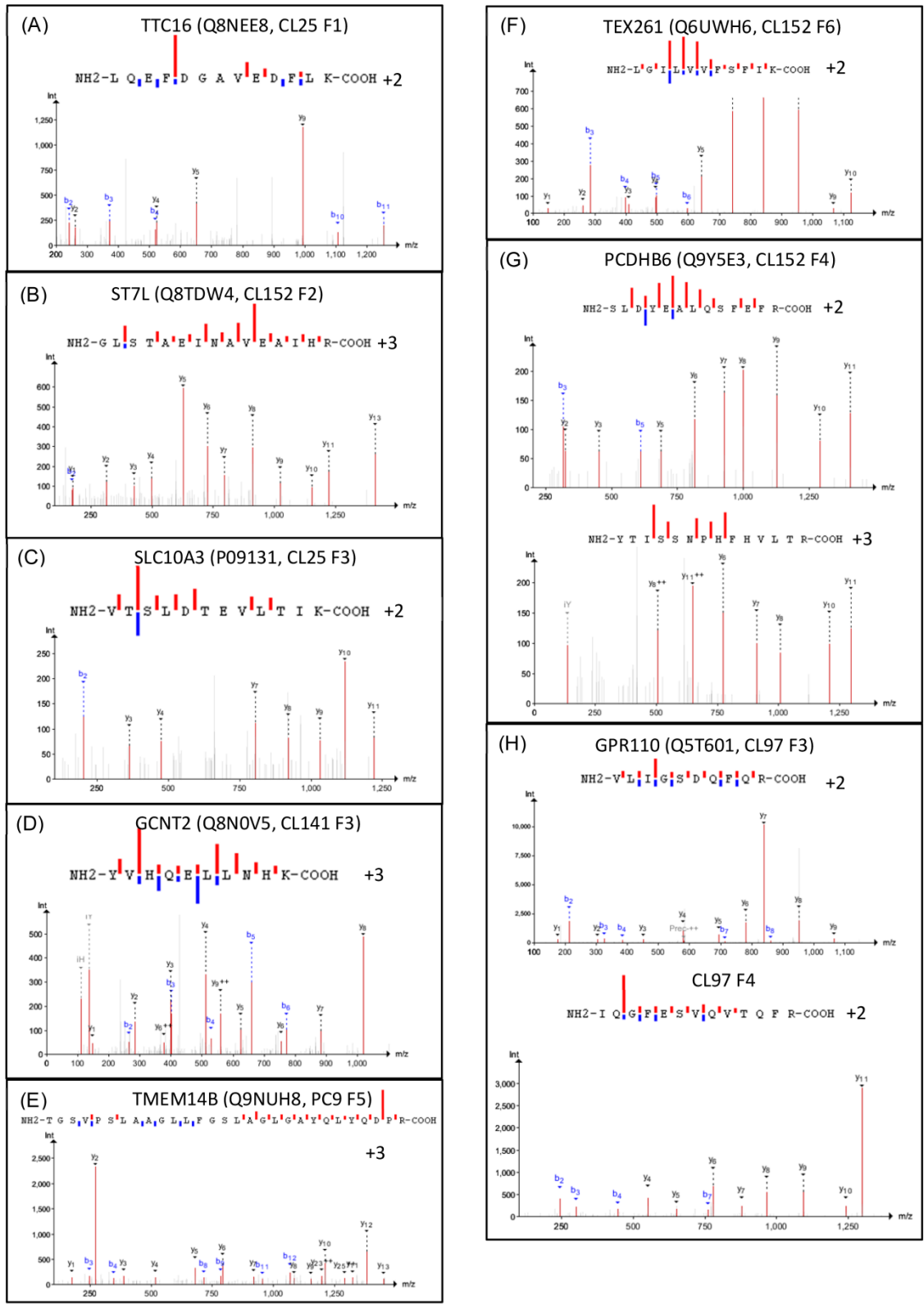
Figure S4. Sample DDA spectra of 8 validated missing proteins. (A) TTC16, (B) ST7L, (C) SLC10A3, (D) GCNT2, (E) TMEM14B, (F) TEX261, (G) PCDHB6, (H) GPR110
