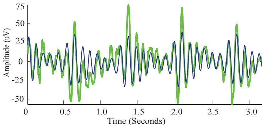
(C) Raw Recording vs. BCG Estimate (Harmonic Regression)
