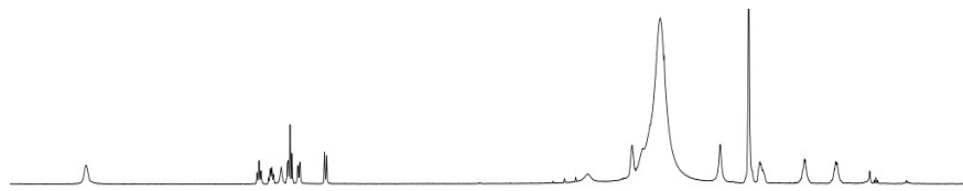
ARN5187 HSQC (DMSO-d6), 300 K, 400 MHz
