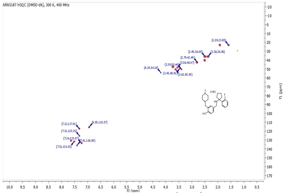
ARN5187 HSQC (DMSO-d6), 300 K, 400 MHz
