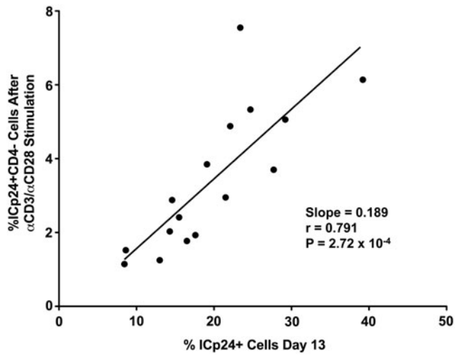
SUPPLEMENTARY FIG. S3. Sixteen separate samples of cultured T_{CM} cells from 10 blood donors were latently infected with HIV-1 NL-43 . On day 13 ICp24 was measured using flow cytometry. On day 19, ICp24 and CD4 were measured by flow cytometry. A linear regression was performed. Slope, Pearson's correlation, and two-tailed p values are shown.
