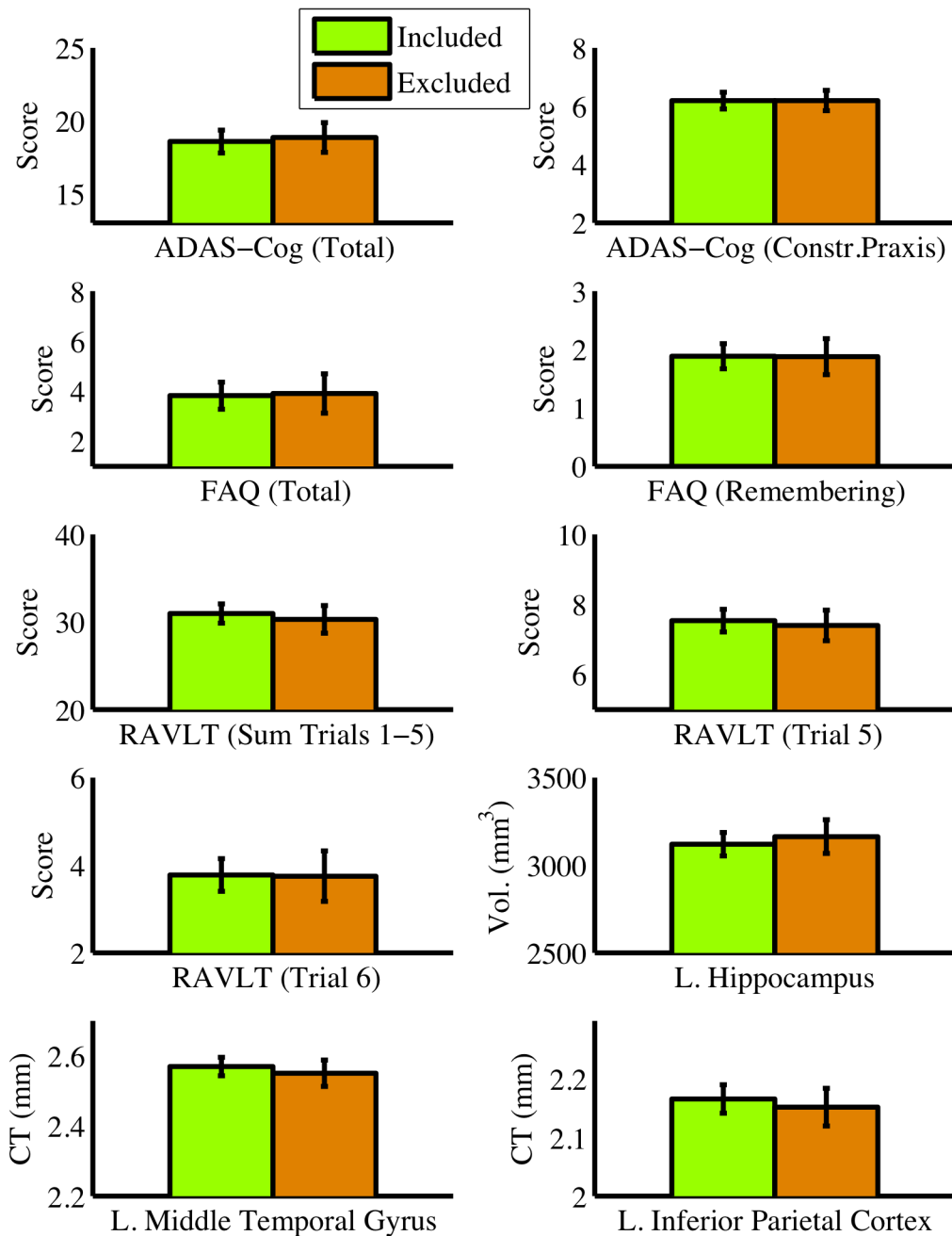
Figure S1. Comparison between included (n=259) and excluded (n=131) MCI subjects on baseline predictor variables. Error bars are 95% confidence intervals. No group differences were found for any of the predictor variables (all P > 0.4 ). Vol. = volume, CT = cortical thickness, ADAS-Cog = Alzheimer's Disease Assessment Scale – Cognitive sub-scale, FAQ = Functional Activities Questionnaire, RAVLT = Rey Auditory-Verbal Learning Test, L. = Left, Constr. = Constructional
