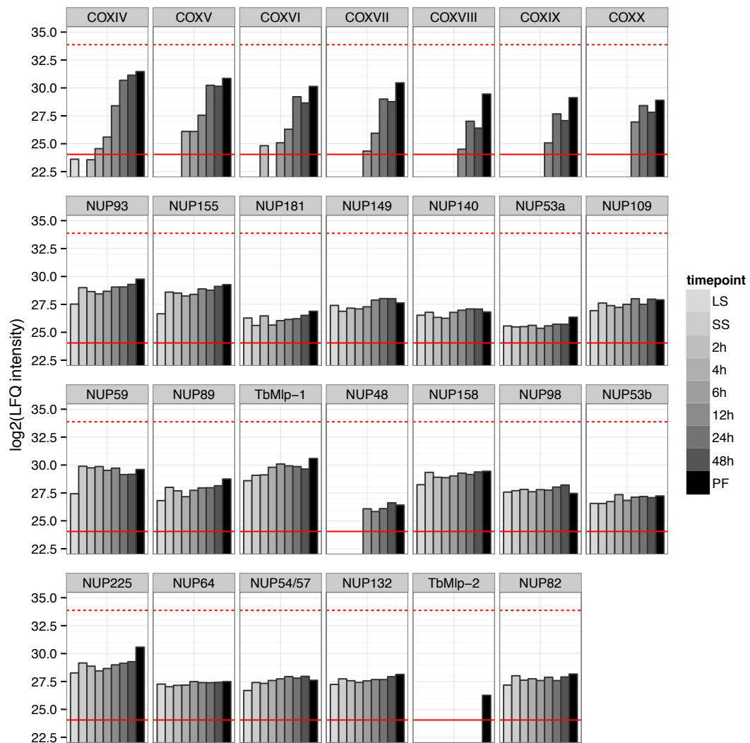
Fig S4: Changes in LFQ intensity of cytochrome oxidase subunits and nuclear pore complex proteins. Log 2 LFQ intensities of proteins are shown for long slender (LS) and short stumpy (SS) forms and consecutive time points during the differentiation as indicated.
