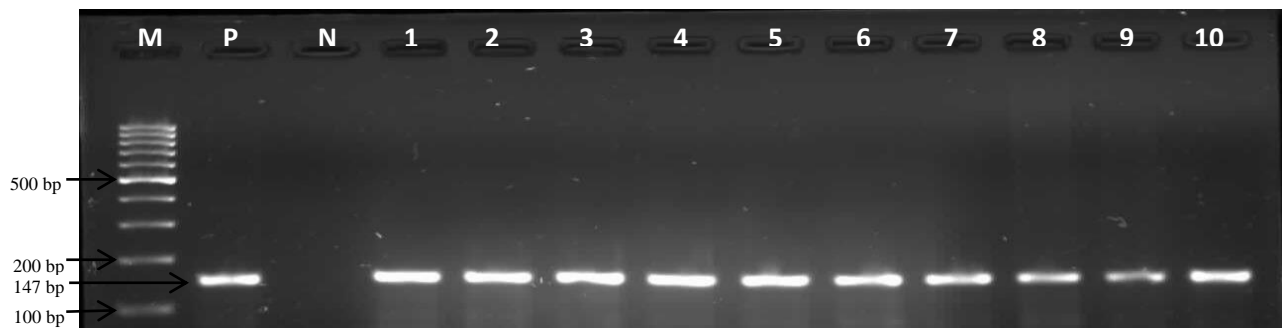
Supplementary Figure 1. Gel electrophoresis image of E. coli identification. Lane M: 100 bp molecular weight marker (Thermo Scientific Inc.); lane P: positive control ( E. coli ATCC 25922 strain); lane N: negative control; lanes 1 to 10 PCR-confirmed E. coli isolates.
