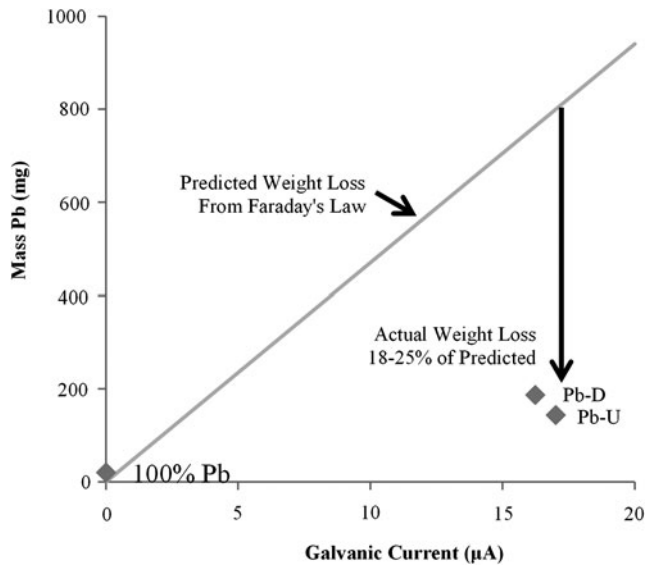
SUPPLEMENTARY FIG. S1. Average weight loss versus average sacrificial current of 10 cm Pb coupon located immediately adjacent to copper pipe versus the estimated weight loss calculated by Faraday's Law.
