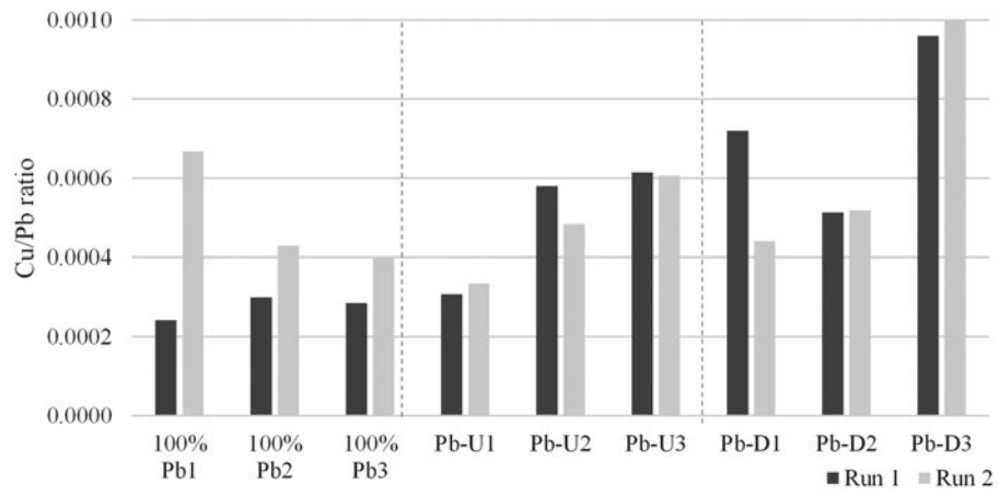
SUPPLEMENTARY FIG. S2. Mass ratio of copper/lead in rust removed from short Pb sections.
