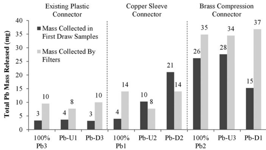
SUPPLEMENTARY FIG. S3. Total mass released in first 2 L draws during prolonged stagnation events during Phase D, months 26–27, and total mass captured by filters during Phase E, months 35–48 (Note: During one sampling period, Rig Pb-U3 malfunctioned, resulting in no flow for a period of 3 months).
