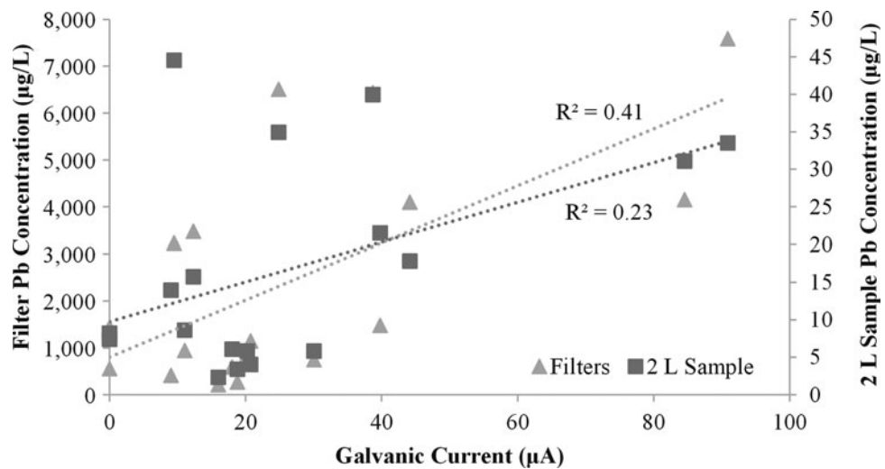
SUPPLEMENTARY FIG. S4. Lead concentration in water collected from both filter samples and 2L draw compared to average galvanic current during that same time period.
