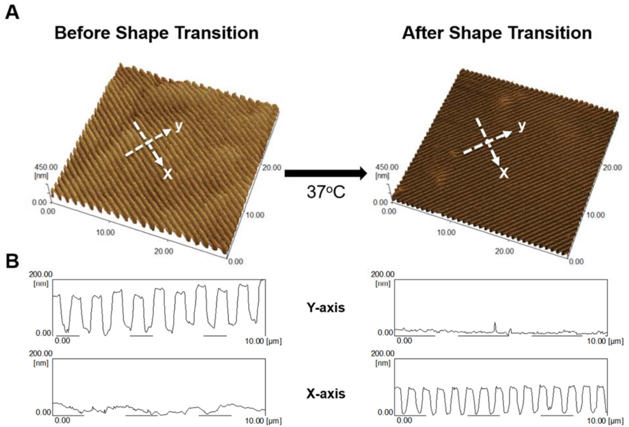
Figure 2: AFM characterization of PCL temporary and permanent topography. (A) Atomic force microscopy image of temporary and permanent topographies after heat-induced shape transition. (B) Cross-sectional profiles of temporary and permanent PCL topography's ridge, groove, and depth in the x- and y-axis direction indicated by arrows in (A).
