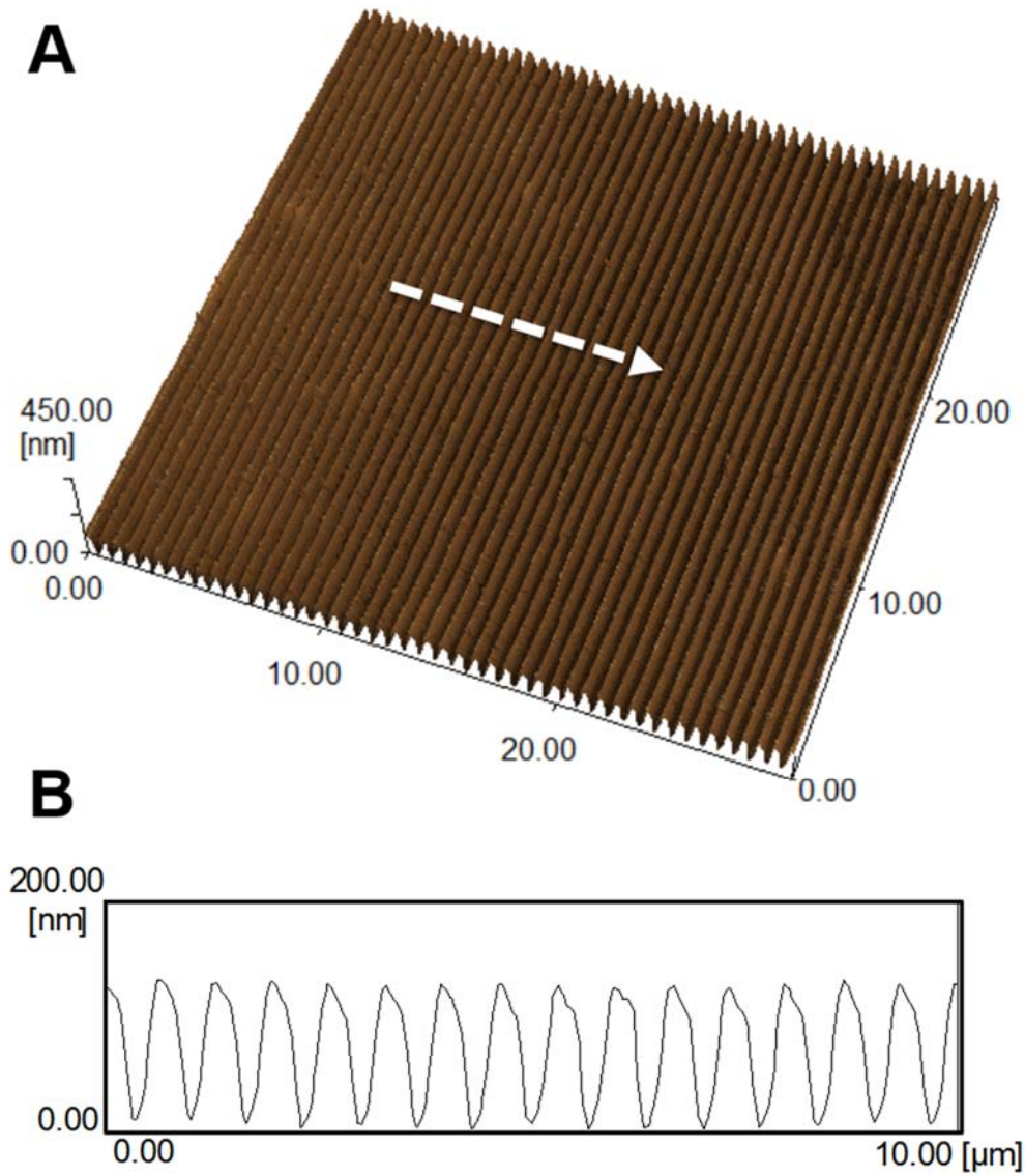
Figure 3: AFM characterization of permanent PCL topography prior to embossing a temporary pattern. (A) Atomic force microscopy image of a permanent PCL topography. (B) Cross-sectional profile of permanent PCL topography's ridge, groove, and depth indicated by arrow in (A).
