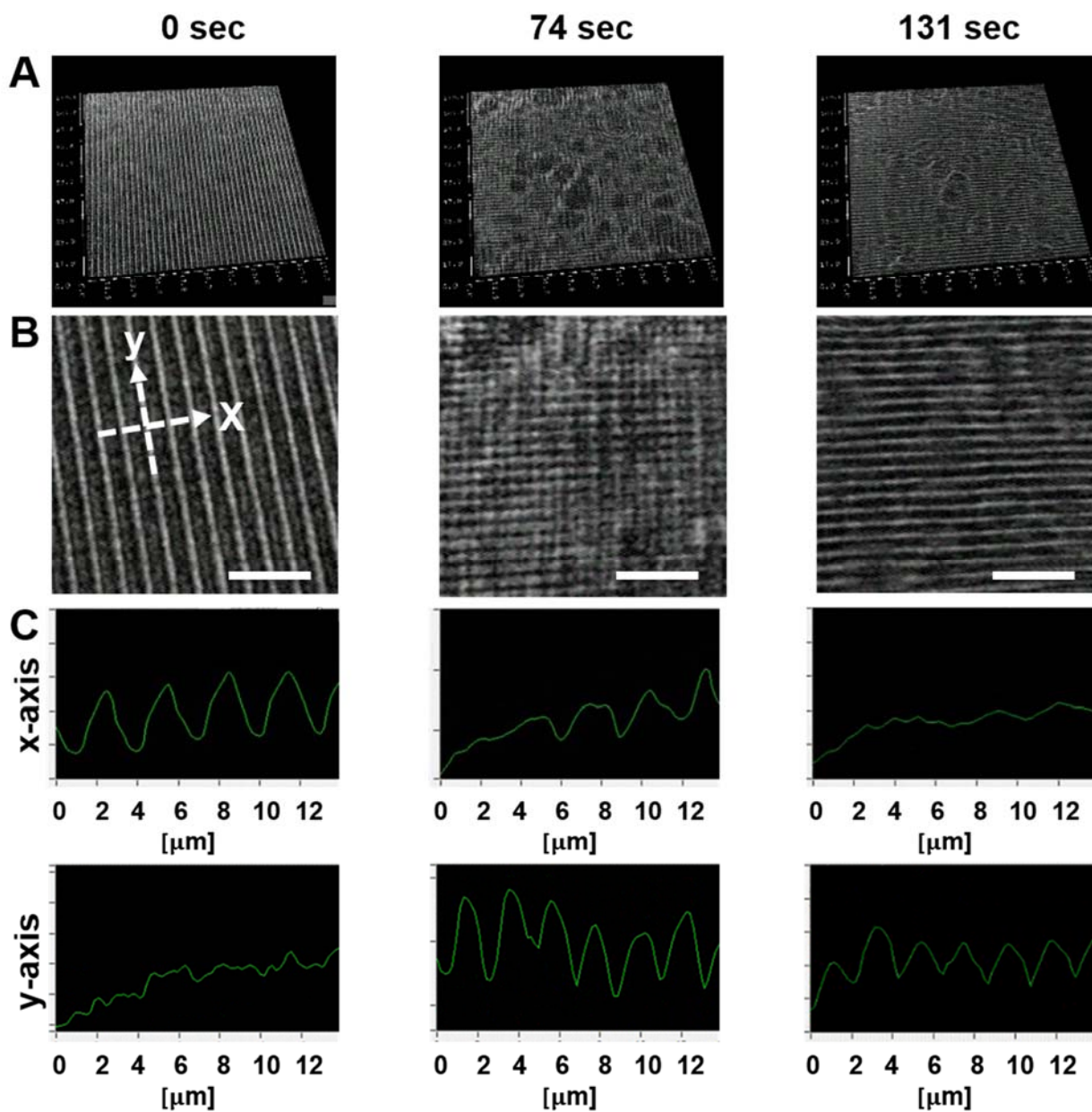
Figure 4: Dynamic holographic microscopy analysis of PCL shape transition. The shape memory polymer's anisotropic topography shifts orientation by 90 degrees during shape transition. (A) Snapshots of PCL topography with 2000_1000_150 nm (groove_ridge_depth) dimensions during shape transition at 0, 74, and 131 seconds. (B) Magnified image of (A) with reference axes for quantifiable analysis of topographic change (scale bar = 10 \mu\text{m} ). (C) The x- and y-axis demonstrate the orthogonal pattern shift over time, with deterioration of topography in the x-axis and development of topography in the y-axis. At 131 seconds a clear shift in topography from the x to the y axis is seen.
