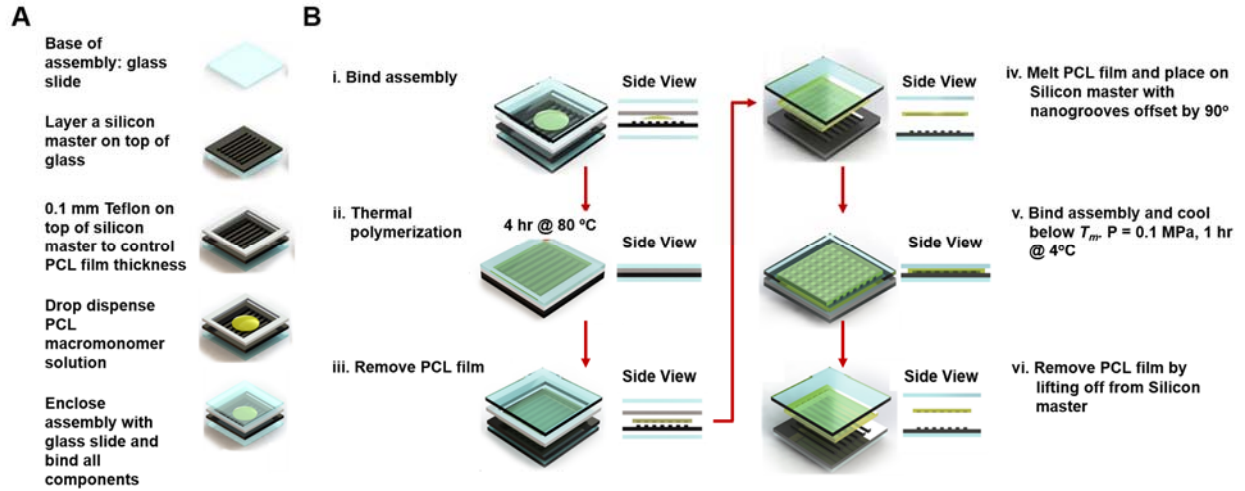
Figure 1: Fabrication of PCL-based shape memory nanogrooves with a temporary and permanent state. (A) During prefabrication assembly, a Teflon spacer is used to control PCL film thickness, and PCL macromonomer solution is sandwiched between a silicon master and glass slides. The assembly is bound (Bi.) and then thermal polymerization takes place at 80°C for 4 hours (Bii.). Then, the PCL film is lifted off with a nanogrooved permanent state (Biii.). Next, a temporary pattern with anisotropic nanogrooves oriented 90 degrees from the permanent state is fabricated. (Biv.) The permanent pattern is melted at 80°C for 2 minutes and then placed on the silicon master with a 90 degree groove offset. It is then bound in between glass slides with a pressure of 0.1 MPa. (Bv.) The assembly is cooled for 1 hour at 4°C, and then the PCL film is lifted off (Bvi.), achieving a PCL-based SMP with a temporary and permanent anisotropic nanogrooved state that are orthogonally offset .
