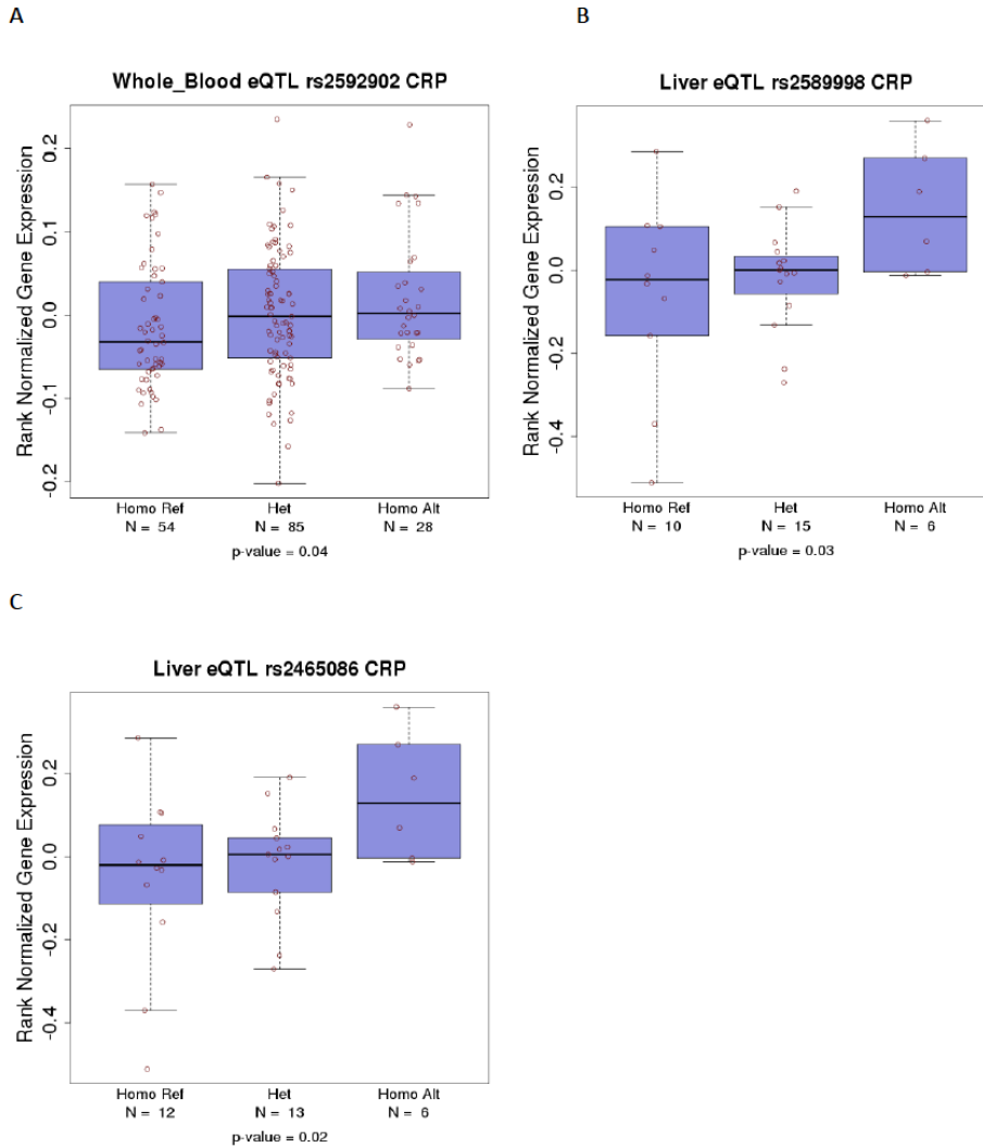
Figure e-3. Expression quantitative trait loci (eQTL) analysis of CRP gene expression.
