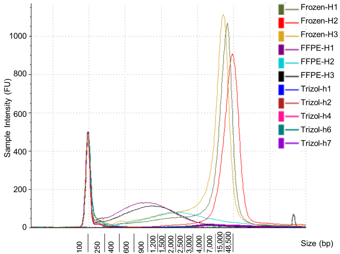
S2 Fig. Fluorescent electropherogram of Frozen-DNA, FFPE-DNA and Trizol-DNA measured by the 2200 TapeStation.
