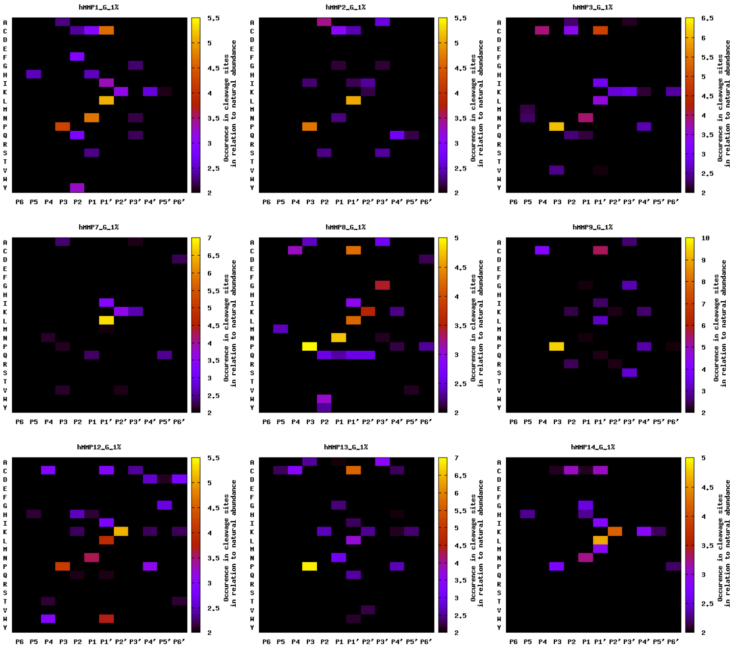
Supplementary Figure 3. Specificity profiles of MMPs 1, 2, 3, 7, 8, 9, 12, 13, and 14 using GluC-generated human peptide libraries. Identified cleavage sites are summarized as heat maps showing fold-change over natural abundance. P6 to P6' subsite positions are shown on the x axes with the identified cleavage site between P1 and P1'. Plotted amino acids are indicated on the y axes with single-letter codes. Please refer to Supplementary Figure 3 for corresponding results using GluC-generated peptide libraries.
