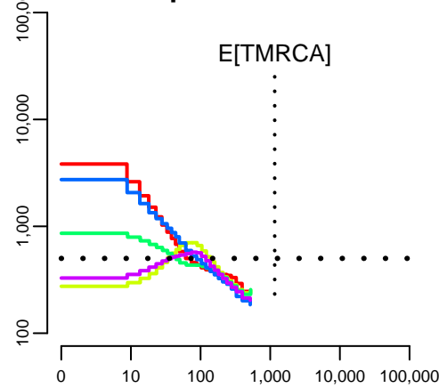
unphased data
