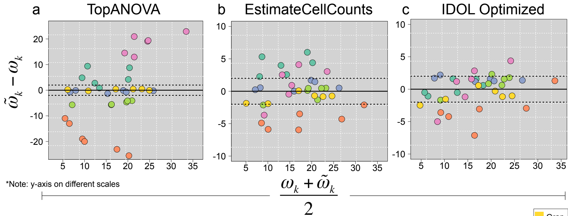
Supplementary Figure 3: Bland-Altman plots constructed from cell fraction estimates of the n = 6 MethodA reconstruction samples obtained using the TopANOVA (a), EstimateCellCounts (b), and IDOL Optimized (c) L-DMR libraries.
