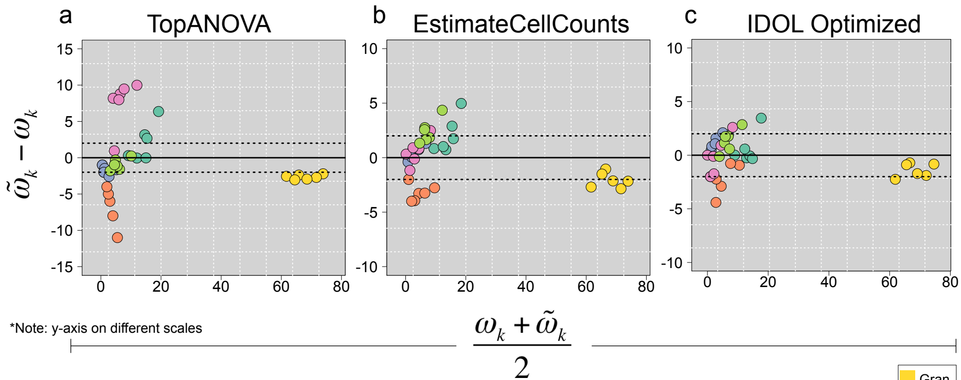
Supplementary Figure 4: Bland-Altman plots constructed from cell fraction estimates of the n = 6 MethodB reconstruction samples obtained using the TopANOVA (a), EstimateCellCounts (b), and IDOL Optimized (c) L-DMR libraries.
