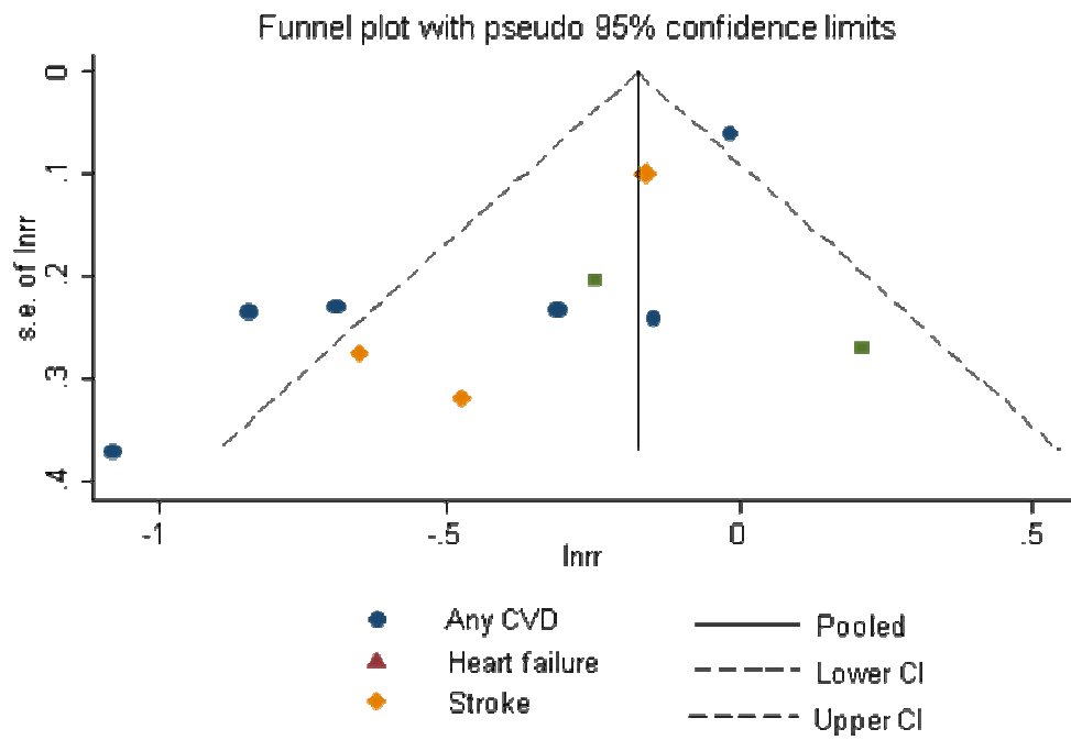
Supplementary figure 1. Funnel plot with 95% confidence limits.
