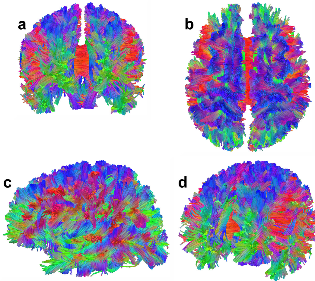
Figure S1: Tractography results of a Radial DSI (4 shells, 59 radial lines) reconstruction of a healthy human brain volunteer acquired using a twice refocused spin echo sequence as seen frontally (a), superiorly (b), laterally (c) and obliquely (d).
