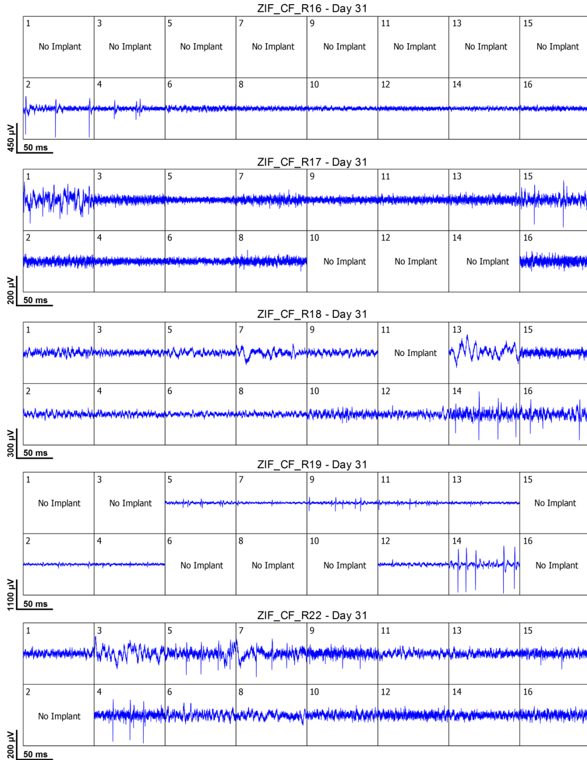
Figure S3. Representative filtered (250 Hz corner, 4 th order Butterworth, high-pass) high speed recordings from each implanted carbon fiber at day 31 post-operatively.
