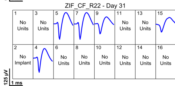
Figure S4. Average waveforms of sorted units detected on each implanted site at day 31 post-operatively.
