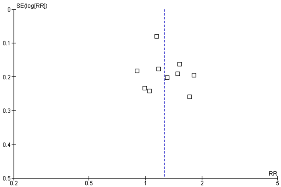
Fig C Funnel plot for baseline impaired glucose tolerance (IGT) or combination of IGT and impaired fasting glucose
