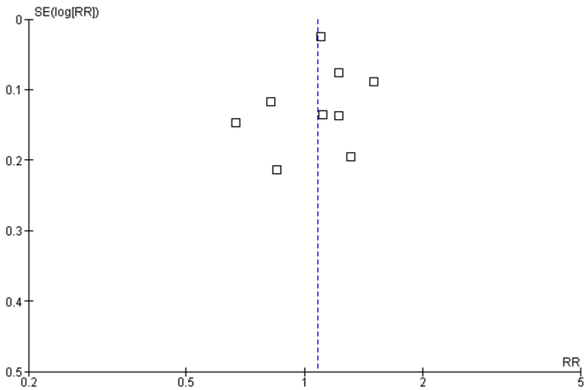
Fig A Funnel plot for baseline fasting glucose 100-125 mg/dL
