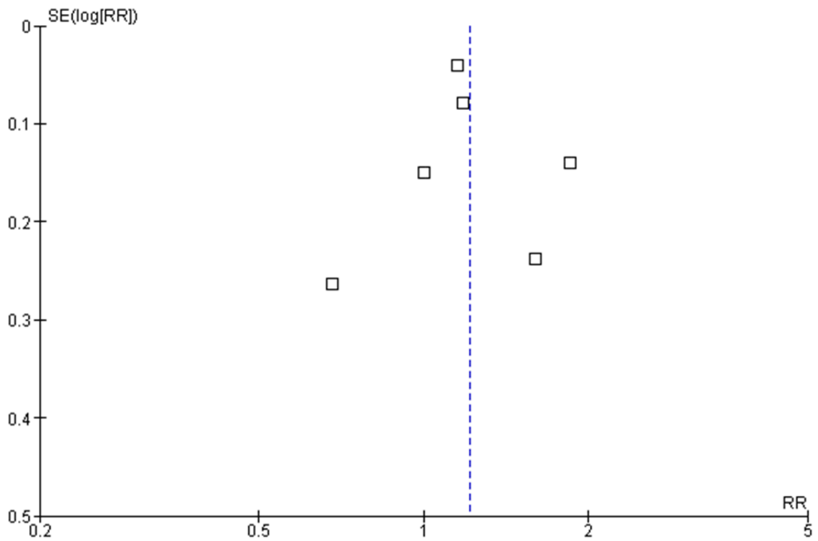
Fig B Funnel plot for baseline fasting glucose 110-125 mg/dL
