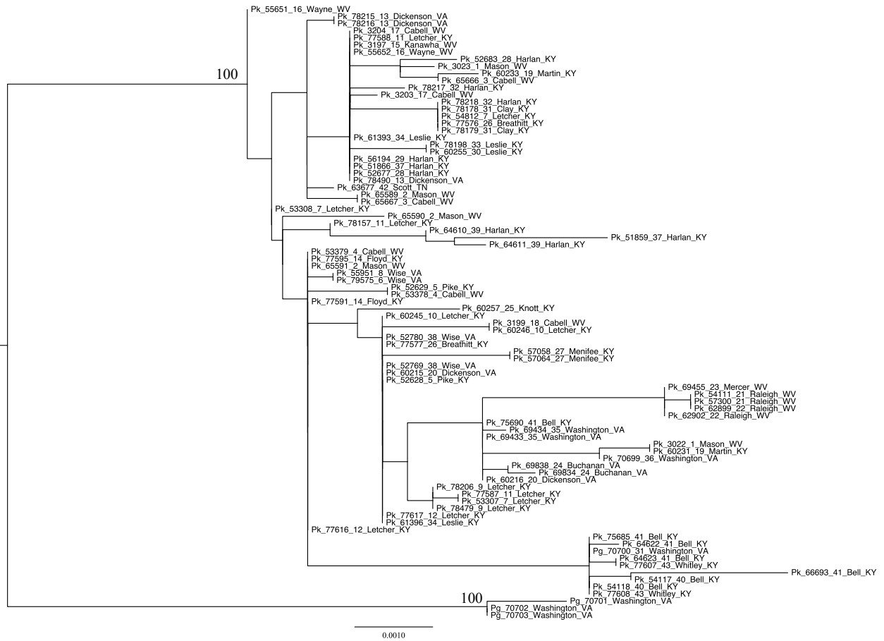
Figure H. Maximum likelihood analysis of the concatenated nuclear DNA data. MtDNA data not included. Analysis done in RAxML.
