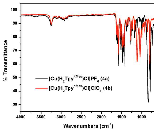
Figure S15: Infrared spectra overlay of 4a and 4b collected on solid samples.
