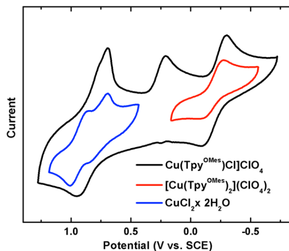
Figure S23: Cyclic voltammograms of 5 , 6 , and free \text{CuCl}_2 in 0.1M \text{TBAClO}_4 \text{CH}_2\text{Cl}_2 showing the presence of both 6 and \text{CuCl}_2 in samples of 5 .
