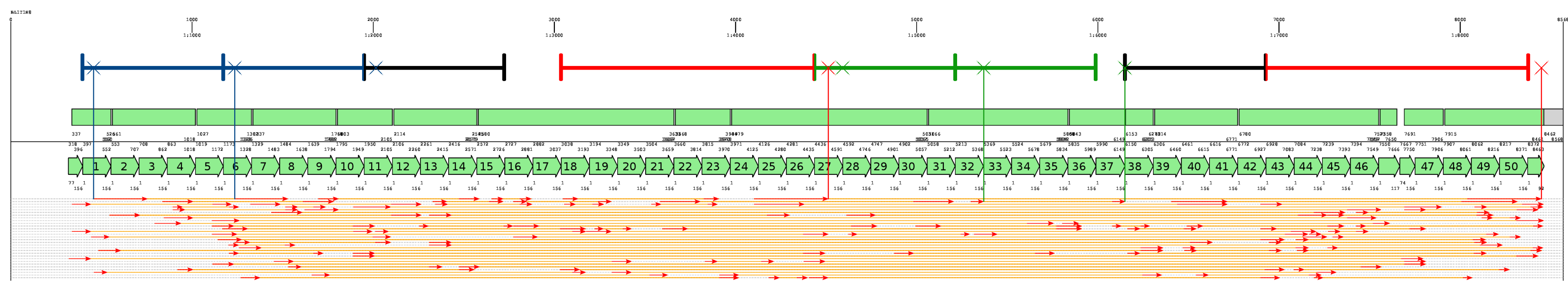
Figure S6. JV image of the B73 CentC array. CentC HORs as defined by full-length CentC monomers are marked above the JV annotations by blue, black, red, and green colored lines as in Figure 6. Alternatively, HOR borders can be defined using the longest MUMmer annotations on the edges of monomer-defined HORs (Xs). The youngest (blue) and oldest (green) HORs date to 131 and 297 kya, respectively. CentC monomers are indicated by green arrows and numbered consecutively as in Figure 6 and Figure S8. The longest perfect matches identified by MUMmer are indicated by red arrows below the numbered CentCs.
