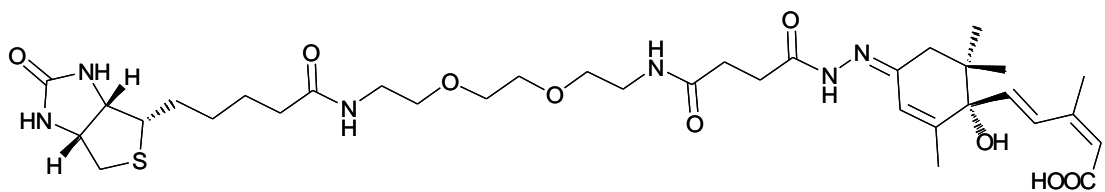
Figure S2. Biotinylated ABA conjugate, b-PEG-ABA. S -(+)-abscisic acid 4'-( N -succinamidyl acyl hydrazide- N' -biotinyl-3,6-dioxaoctane-1,8 diamine). Enantiopure (+)-ABA was conjugated to biotin through C-4' via a 15-atom PEG linker ( b-PEG-ABA ).
