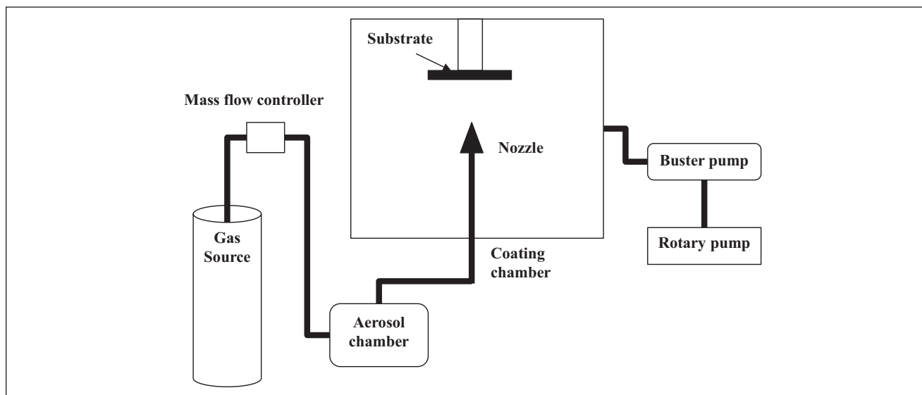
Appendix Figure. Schematic of the aerosol deposition process.
