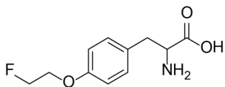
O-(2-Fluoroethyl)-L-tyrosine (FET)
