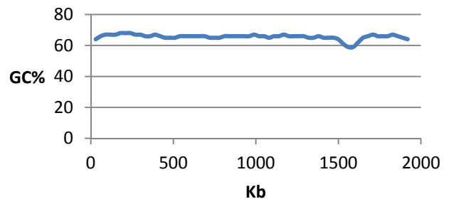
RCC299 Chromosome 2 GC%
