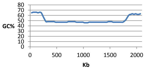
RCC299 Chromosome 1 GC%
