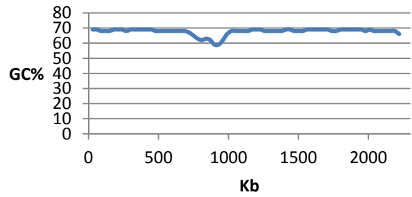
CCMP1545 Chromosome 1 GC%
