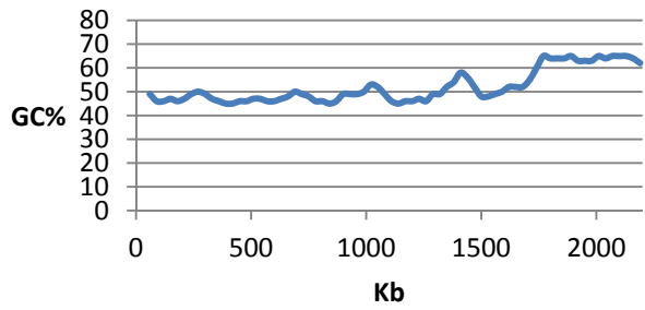
CCMP1545 Chromosome 2 GC%
