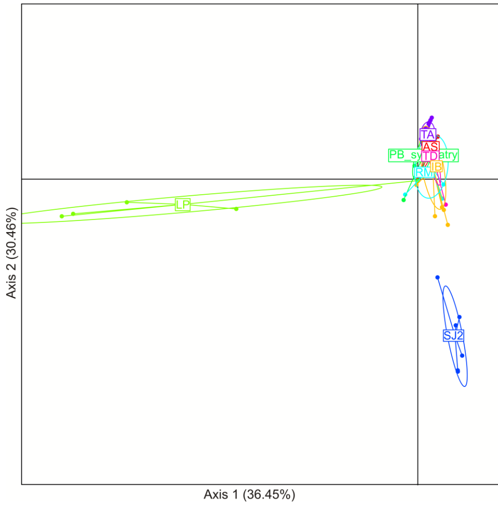
Figure S2. Plot of between-class analysis for the samples of C. flamarioni by sampling site. Locality abbreviations correspond to those in Table 1.
