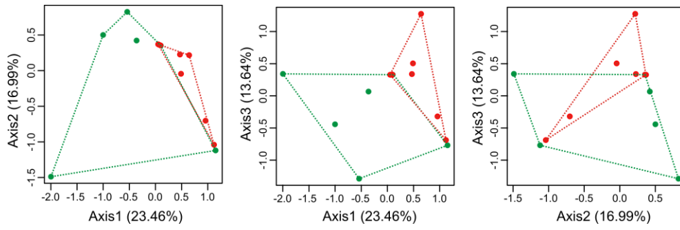
Figure S3. Plots of correspondence analysis for the samples of C. minutus (green dots) and C. flamarioni (red dots) collected in the sympatric region.
