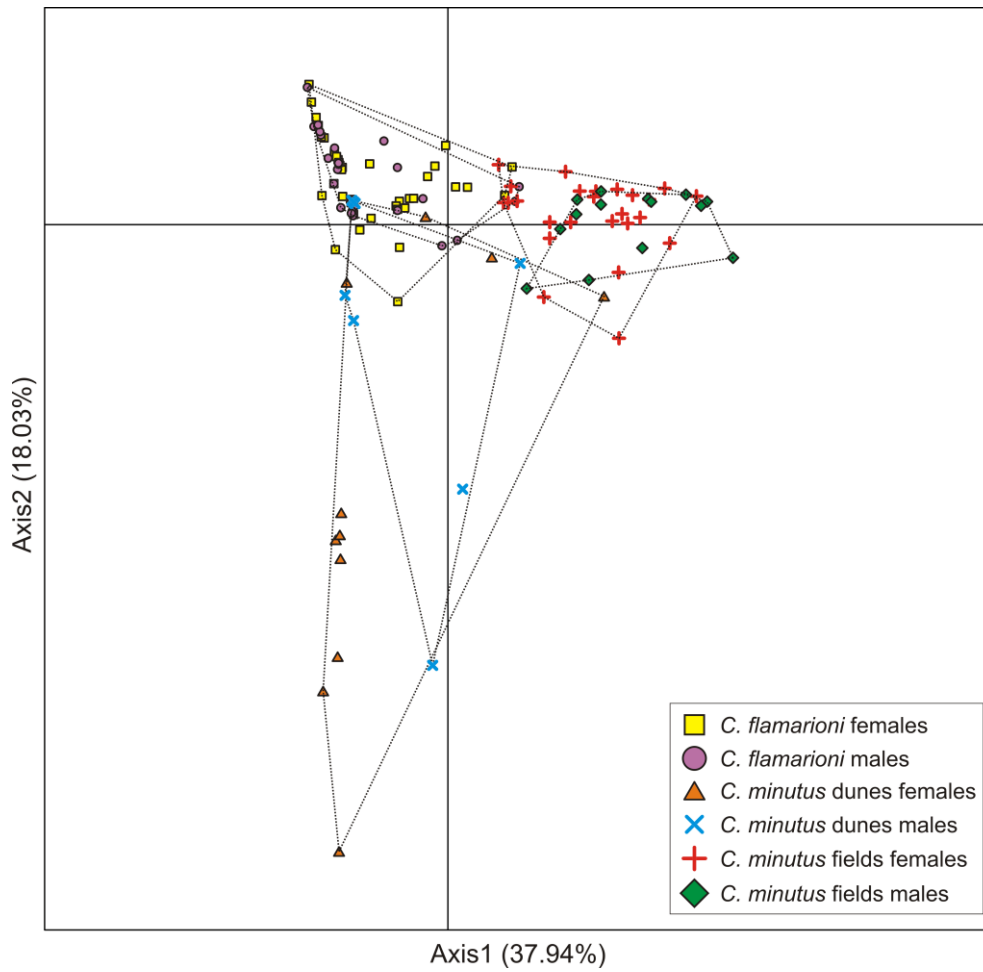
FigureS4. Plot of between-class analysis for samples of male and female individuals for each species in different habitats.
