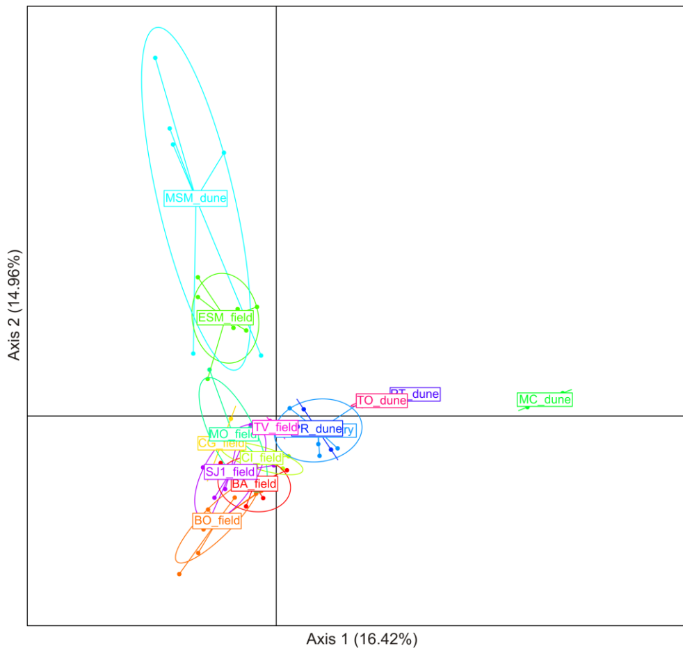
Figure S1. Plot of between-class analysis for the samples of C. minutus by sampling site. Locality abbreviations correspond to those in Table 1.
