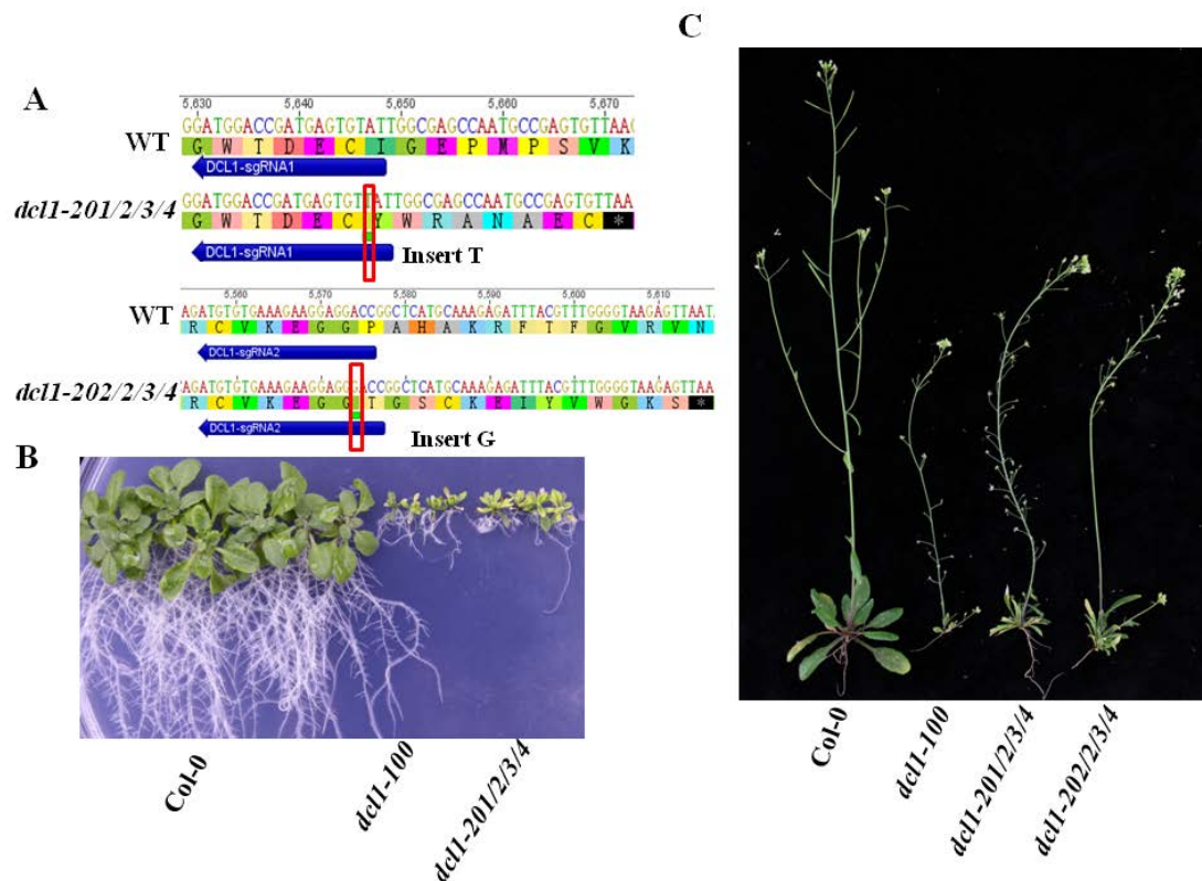
Figure S4 Introducing dcl1 mutations in the dcl2/3/4 mutant. (A) Diagram showing the sequence of sgRNAs and the 1-nt insertion generated in dcl1-201/dcl2/3/4 and dcl1-202/dcl2/3/4 mutants. (B) Phenotype of dcl1-201/dcl2/3/4 seedlings grown on \frac{1}{2} MS nutrient agar plates resembles that of dcl1-100 . (C) Adult dcl1/2/3/4 plants exhibit similar but slightly milder developmental defects compared to dcl1-100 .
