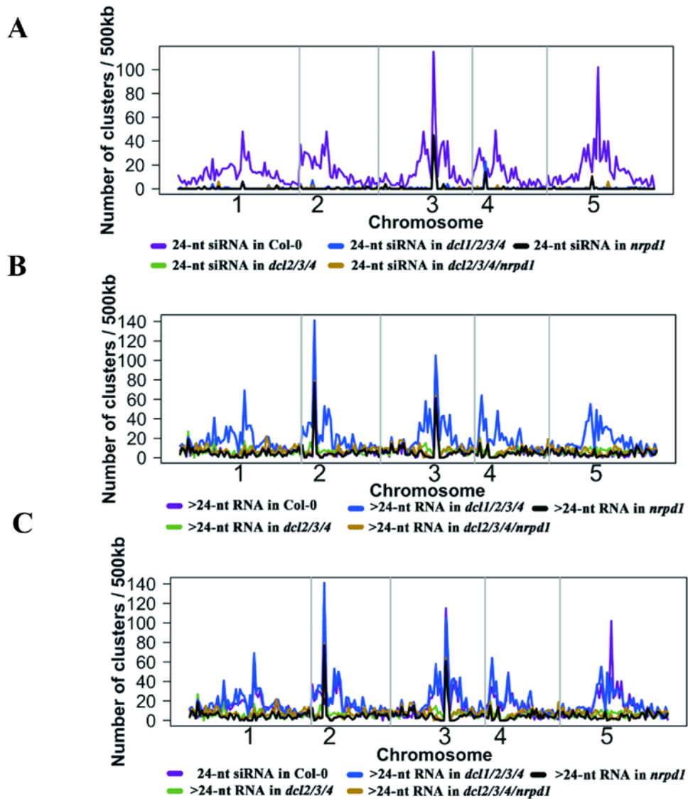
Figure S6 The distribution of 24-nt and >24-nt RNAs on the genome. (A) The distribution of 24-nt siRNA clusters on 5 chromosomes in WT, dcl2/3/4 , dcl1/2/3/4 dcl2/3/4/nprp1 and nprp1 plants. (B) The distribution of >24-nt RNA clusters on 5 chromosomes in WT, dcl2/3/4 , dcl1/2/3/4 , dcl2/3/4/nprp1 and nprp1 plants. (C) The comparison of the distribution of 24-nt RNA clusters in WT and >24-nt RNA clusters in dcl2/3/4 , dcl1/2/3/4 , dcl2/3/4/nprp1 and nprp1 mutants.
