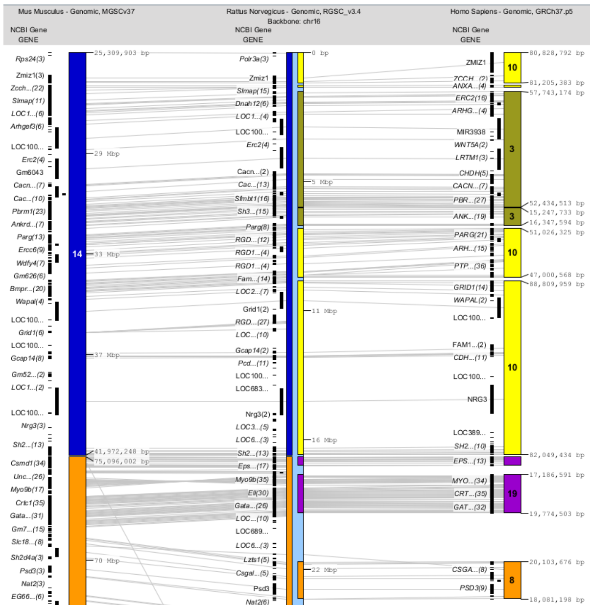
S1 Fig. The comparative map of the differential segment in SHR.BN16 congenic rat showing the correspondence between rat chromosome 16 (center) and the syntenic regions of the murine (left) and human (right) genomes. The figure is generated using the Virtual Comparative Map software tool ( http://www.animalgenome.org/VCmap/ ).
