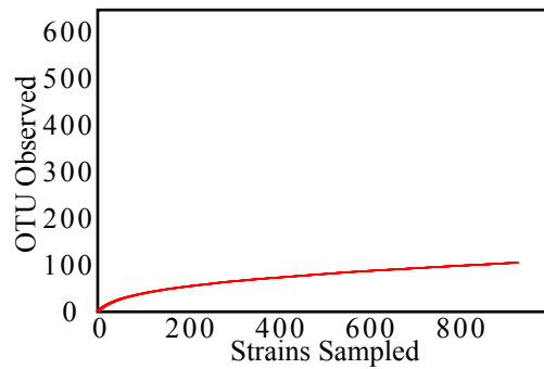
Figure S2. The rarefied collectors curve indicates that OTU rpoB have been well sampled from the sampling sites (with respect to the constraints imposed by strain collection). Good's coverage is 0.88 for unique rpoB sequences and 0.95 for OTU rpoB .
