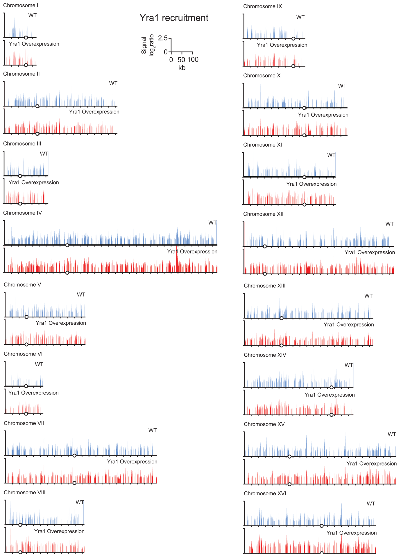
S5 Figure. Genomic view of Yra1 recruitment under Yra1 wild-type (HA-YRA1) and Overexpression (HA-YRA1 \Delta ) conditions. A representation of each chromosome with the signal \log_2 ratio values for the significant ChIP-chip clusters is plotted. The X-axis shows chromosomal coordinates in kb. Positions of centromeres are indicated as open circles.
