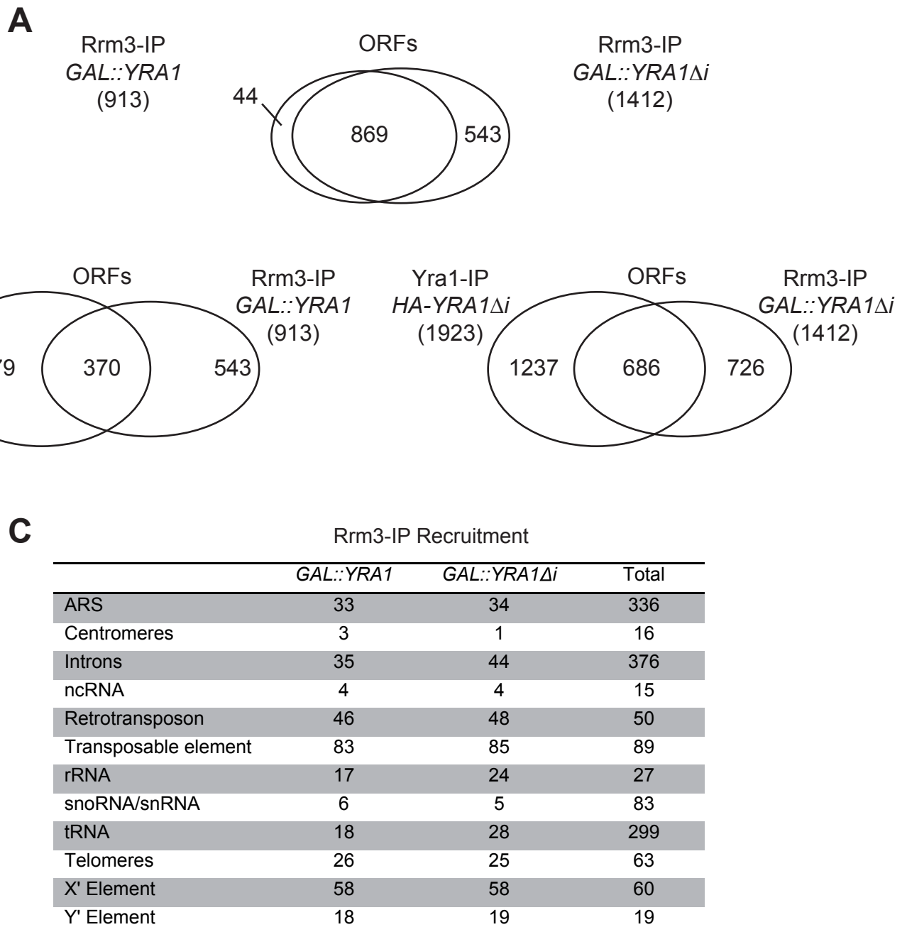
S12 Figure. (A) Venn diagrams showing the overlap between genes with significant Rrm3 binding in the different ChIP-chip experiments. (B) Venn diagrams showing the overlap between genes with significant Yra1 and Rrm3 binding in different ChIP-chip experiments. (C) Rrm3 cluster distribution at ARSs, centromeres, introns, ncRNA, transposable elements, RNAPIII genes, snoRNA/snRNA and telomeres under wild-type ( GAL::YRA1 ) and Overexpression ( GAL::YRA1Δi ) conditions.
