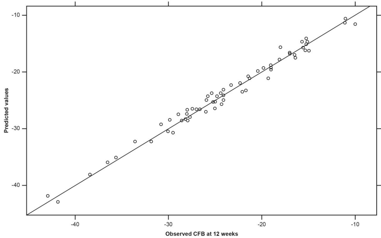
Figure S6: Precision weighted - Random Intercept model: CFB 6 vs. CFB 12 weeks observed vs predicted values and standardized residuals
