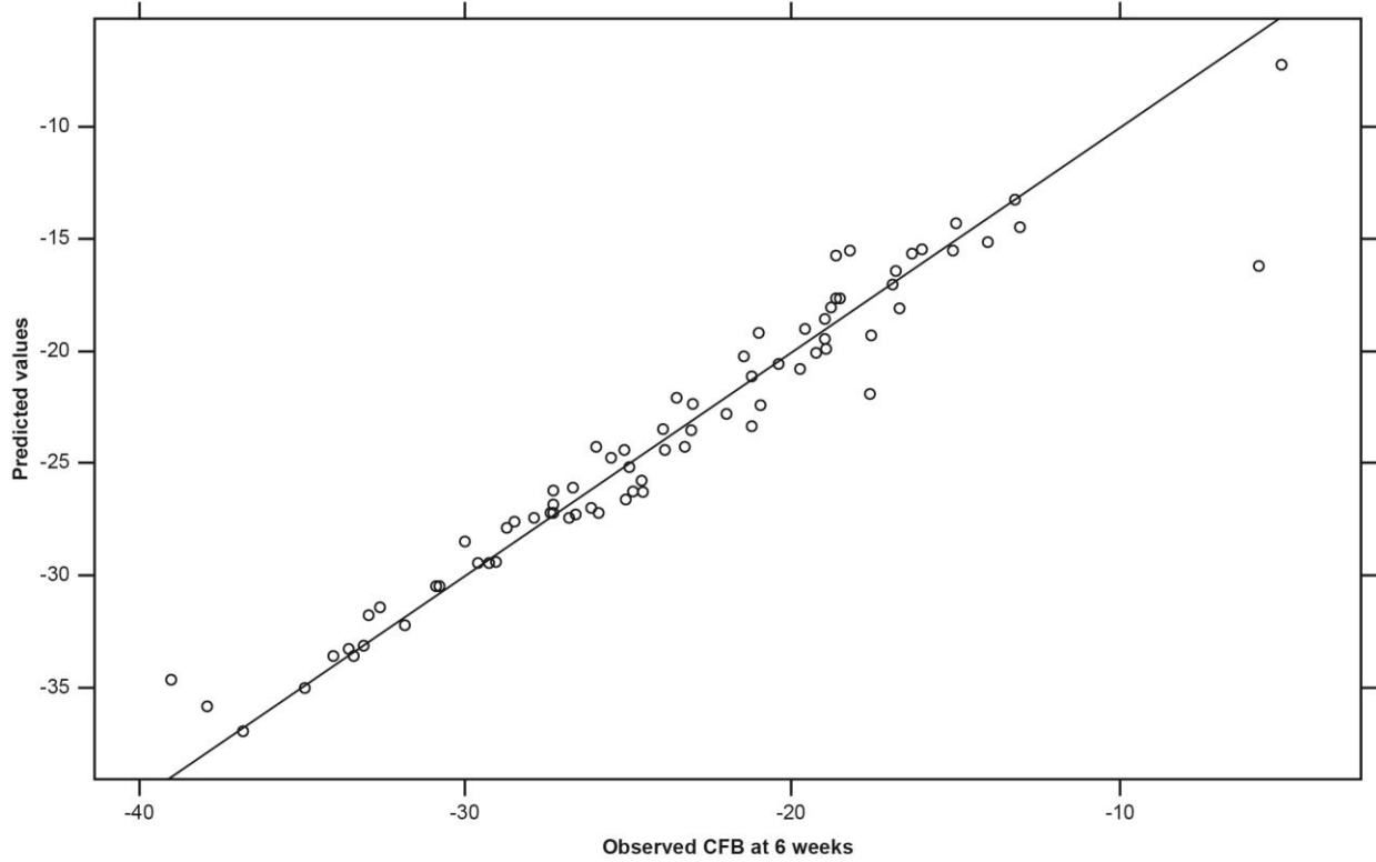
Figure S1: N weighted - Random Intercept model: CFB 2 vs. CFB 6 weeks observed vs predicted values
