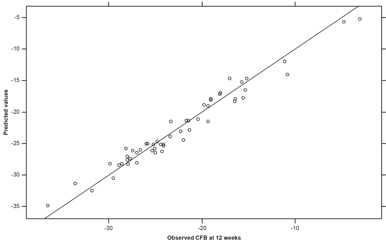
Figure S3: N weighted - Random Intercept model: CFB 2 vs. CFB 12 weeks observed vs predicted values and standardized residuals
