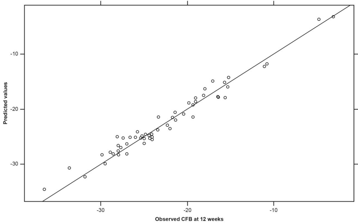
Figure S4: Precision weighted - Random Intercept model: CFB 2 vs. CFB 12 weeks observed vs predicted values and standardized residuals
