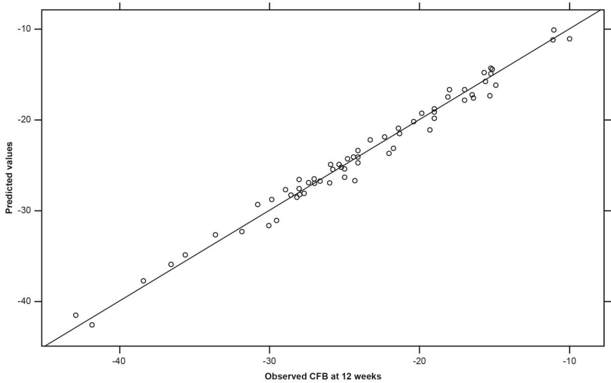
Figure S5: N weighted - Random Intercept model: CFB 6 vs. CFB 12 weeks observed vs predicted values and standardized residuals
