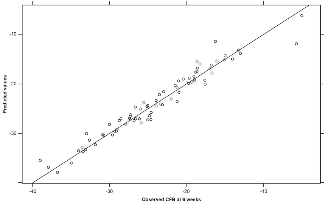
Figure S2: Precision weighted - Random Intercept model: CFB 2 vs. CFB 6 weeks observed vs predicted values and standardized residuals
