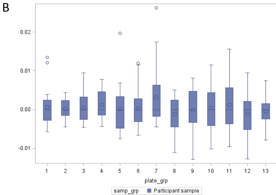
Supplementary Figure 1. Batch effects in the discovery set and their correction. Box-whisker plots of the integrals for glycan Hex 5 HexNAC 4 Fuc 1 by batch number prior to batch corrections (A) and after batch corrections (B). Intensity signals of the standard QC samples included in the batches are also depicted in (A).
