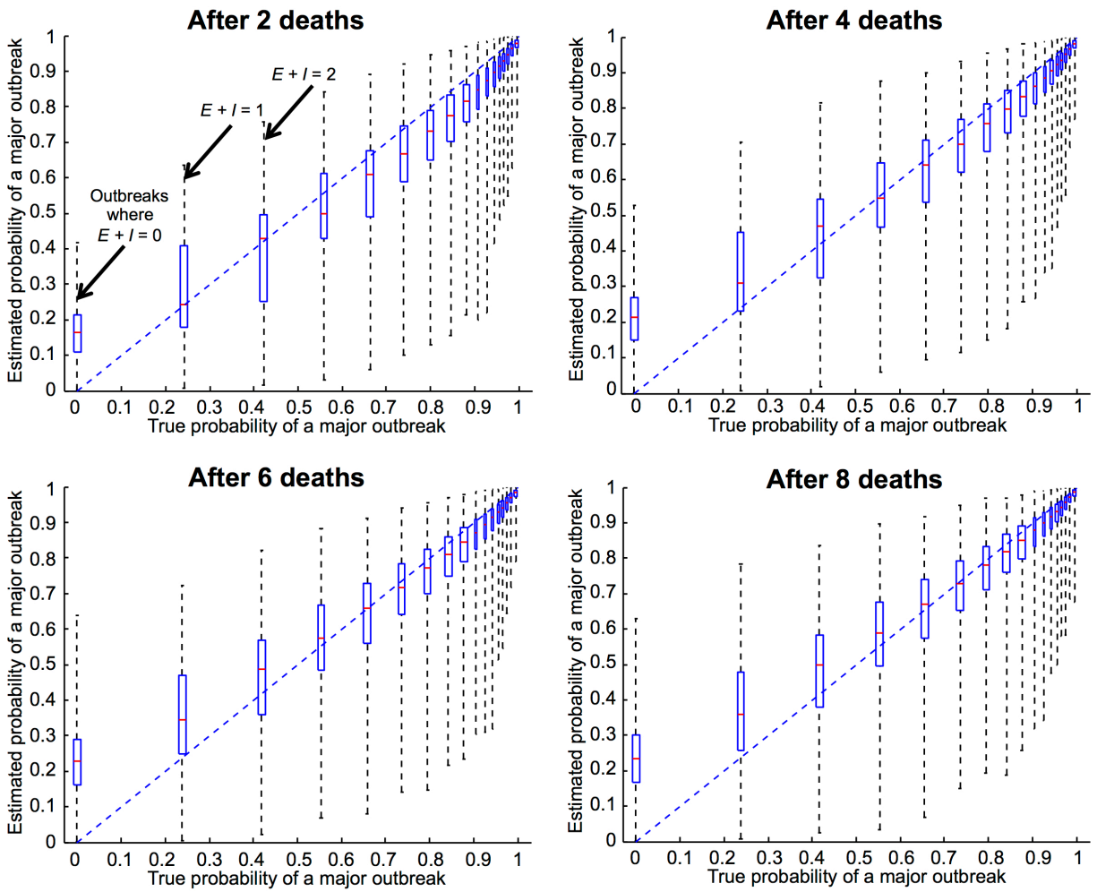
S3 Fig. Robustness of results to different numbers of deaths at the time of estimation. For clarity, true probabilities greater than 0.97 are classified into bins of size 0.01.
