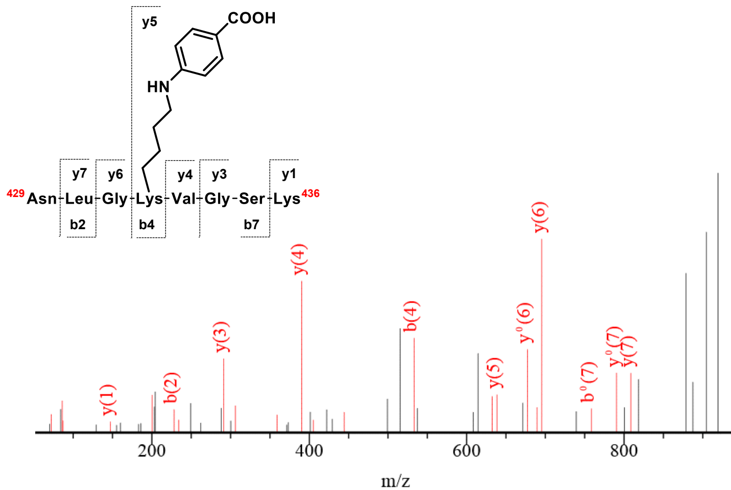
Fig. S7. MS/MS spectrum of the ABA-AAS-containing HSA peptide.
