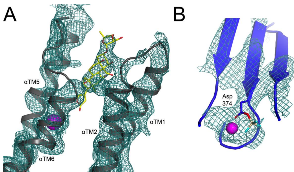
Figure S1 Simple composite omit map (blue mesh) around A ) the ouabain binding site located at the extracellular side of the \alpha TM domain (in gray) shown at 1.5 r.m.s.d. and B ) at the \text{BeF}_3^- substituted phosphorylation site of Asp374 located in the P-domain shown at 3.5 r.m.s.d.. Magnesium ions are shown in magenta spheres.
