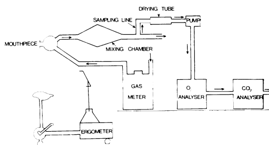
Fig. 1 Circuit diagram of the exercise equipment.
