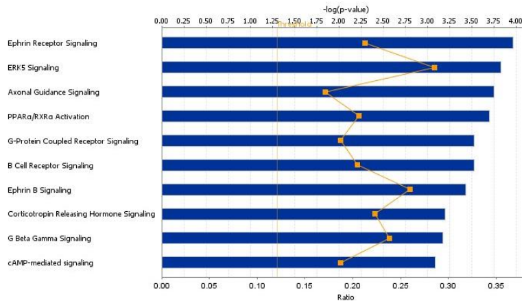
Figure S3. Top ten IPA canonical pathways for putative targets of miRs -4704-3p, -4743, and -4657. Threshold was set at p < 0.05 .
