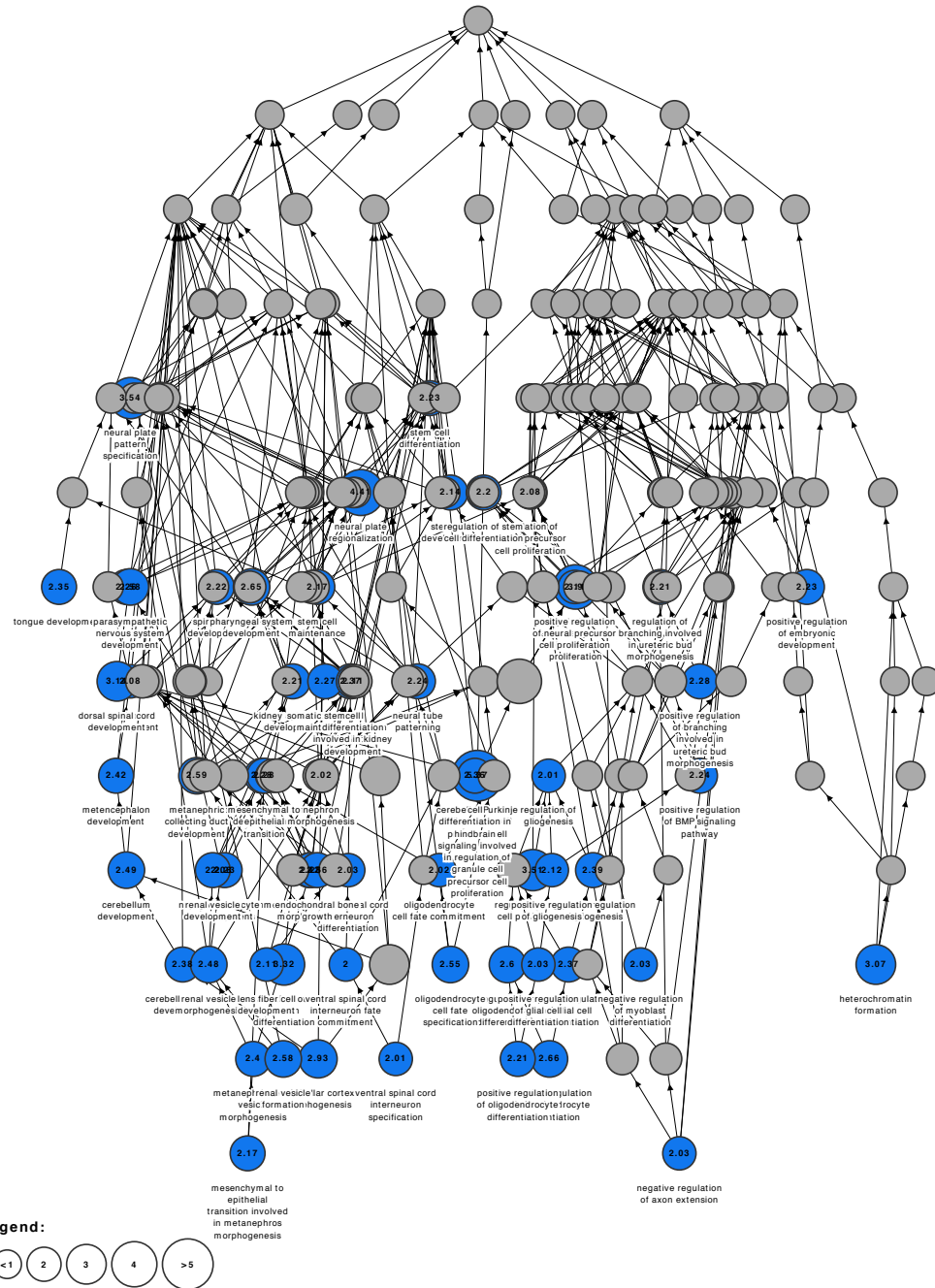
Figure S7. Hierarchy of functional enrichment of genes near hypomethylated VMRs in fetal brain.
