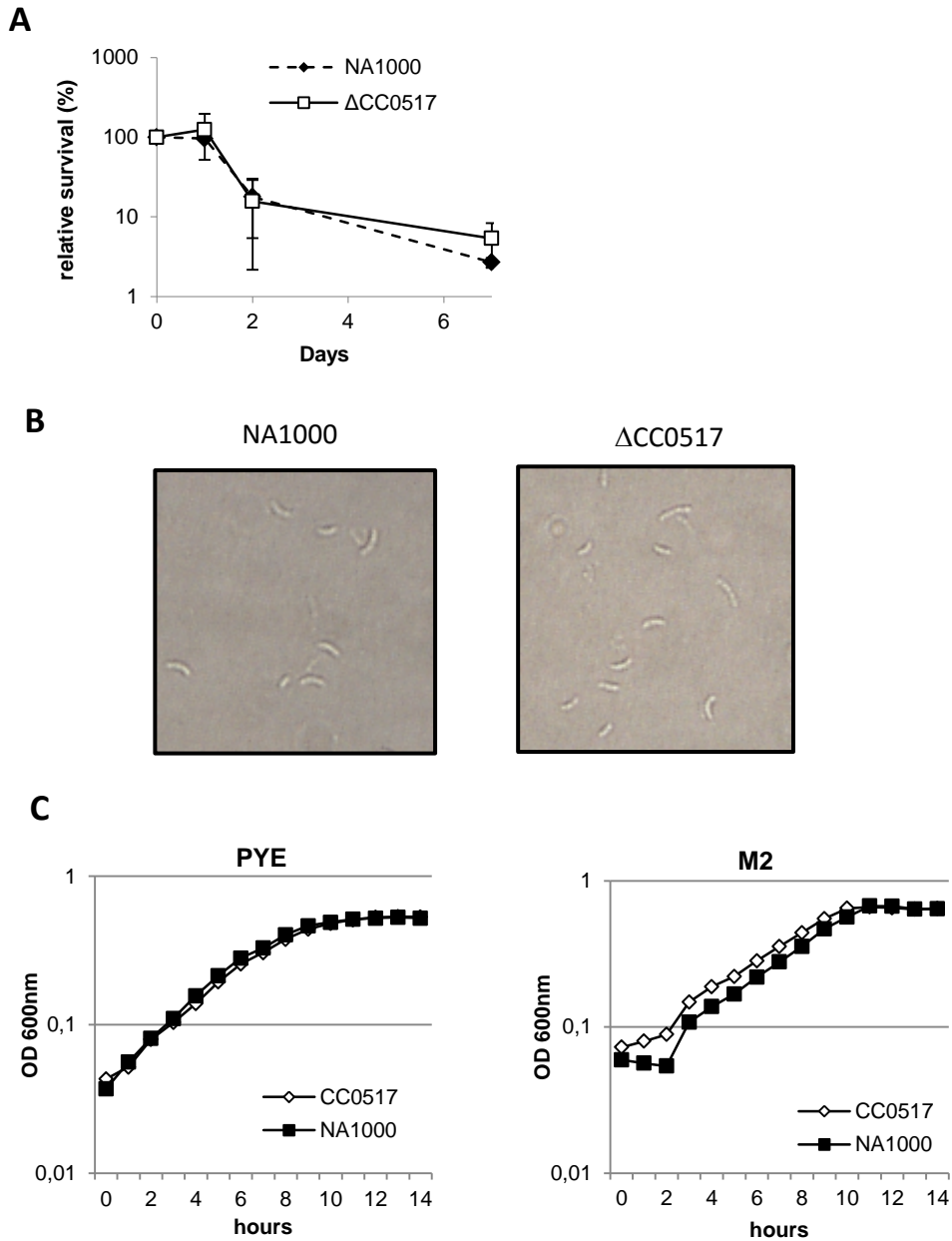
Figure S2. Phenotypic analysis of MM80 ( \Delta CC0517) strain. A. Viability assay of NA1000 and \Delta CC0517 strains at stationary phase in PYE. CFU counts for each time point were determined and the percentage of viability is shown relative to CFU number in exponential phase for the respective strain (day zero). Data represent the means from three experiments in triplicate, with bars indicating the standard error. B. Morphological analysis of NA1000 and \Delta CC0517 strains at early stationary phase (24h). C. Growth curves of NA1000 and \Delta CC0517 strains in PYE and M2 media.
