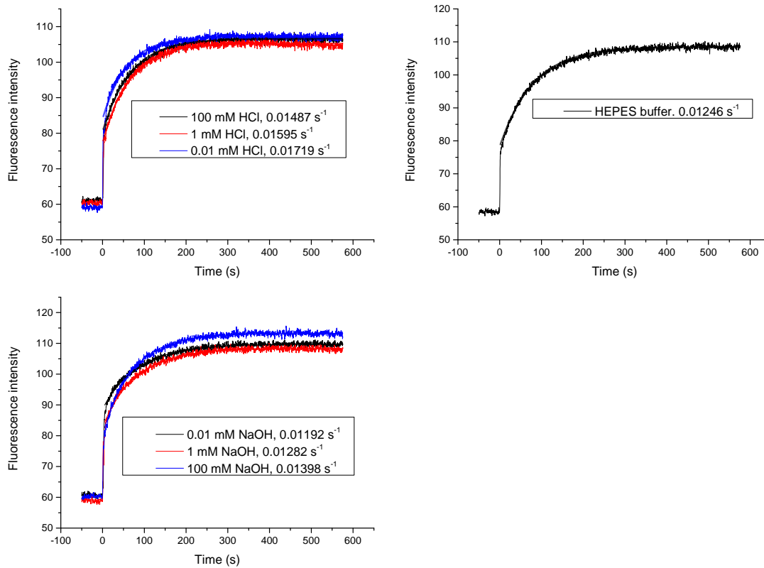
S2 Fig. Fluorescence intensity time courses of Cyp18 upon the addition of CsA dissolved in different pH under continuous stirring.
