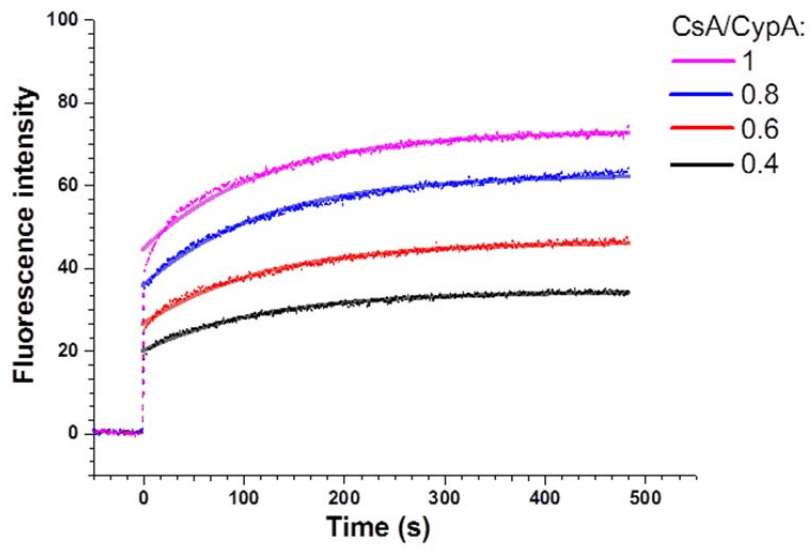
S3 Fig. First order global fitting when CsA was not more than CypA. The values shown in the inset represent the different ratios of CsA to CypA. The k value was 8.25 \pm 0.03 \text{ s}^{-1} .
