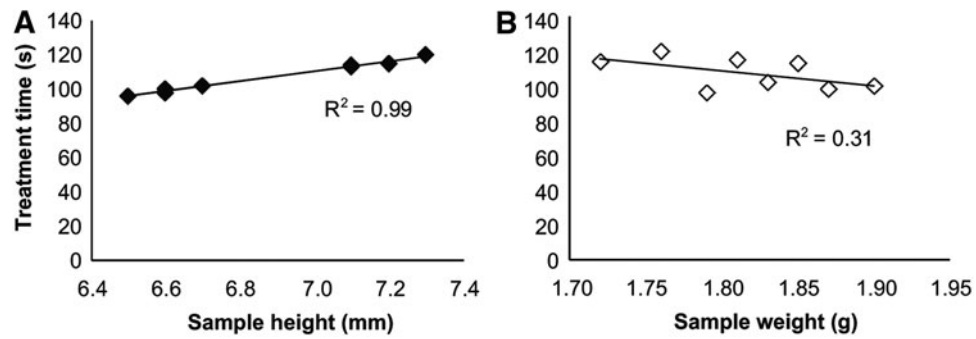
SUPPLEMENTARY FIG. S1. The sample height (A) and weight (B) in relation to treatment time in the Stabilizer T1 instrument. The graphs are based on eight individuals and the treatment time, sample height, and weight are expressed as seconds (s), millimeter (mm), and grams (g), respectively.
